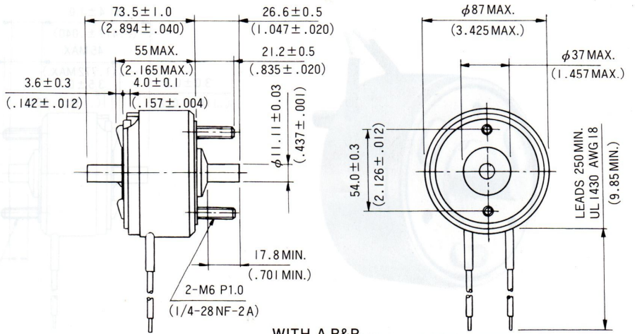
WITH A,B&R
